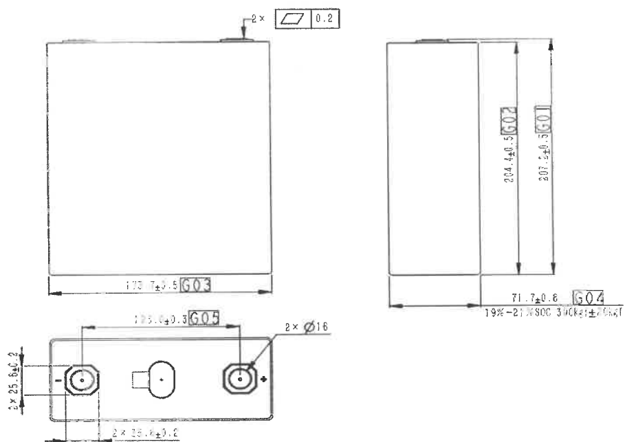
Fig.7 Diagram of Cell Size and Appearance
